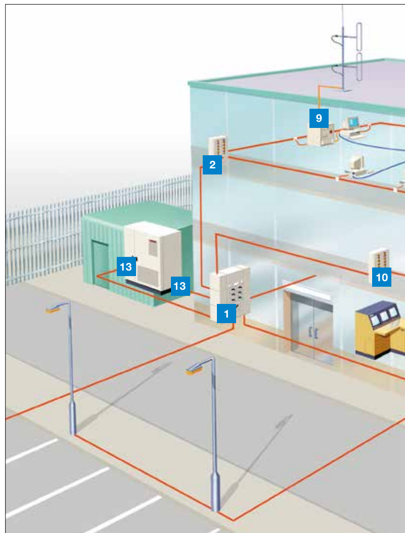
Main aspects and individual components of a system of surge protection methods
